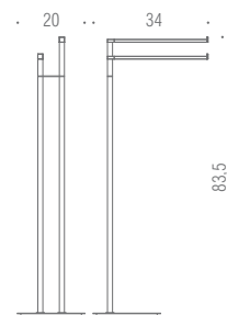
B5038 Piantana con due porta salvietta Standing column with two towel holders
